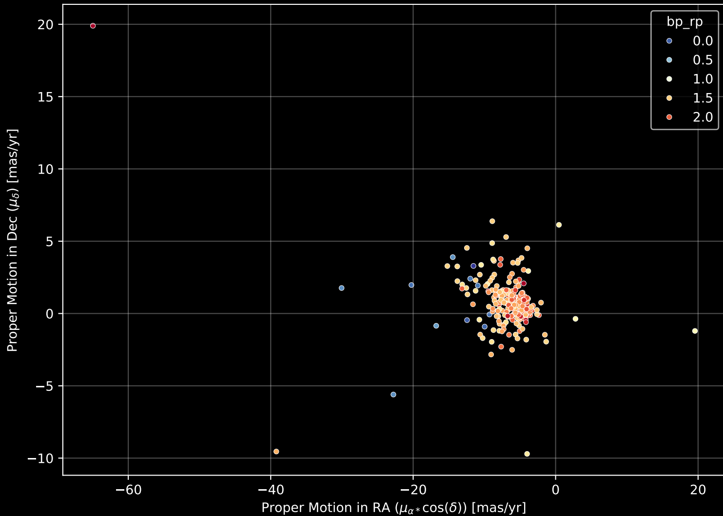
APOGEE DR17 Field: [296+06] Proper Motion Diagram (n= 261)
