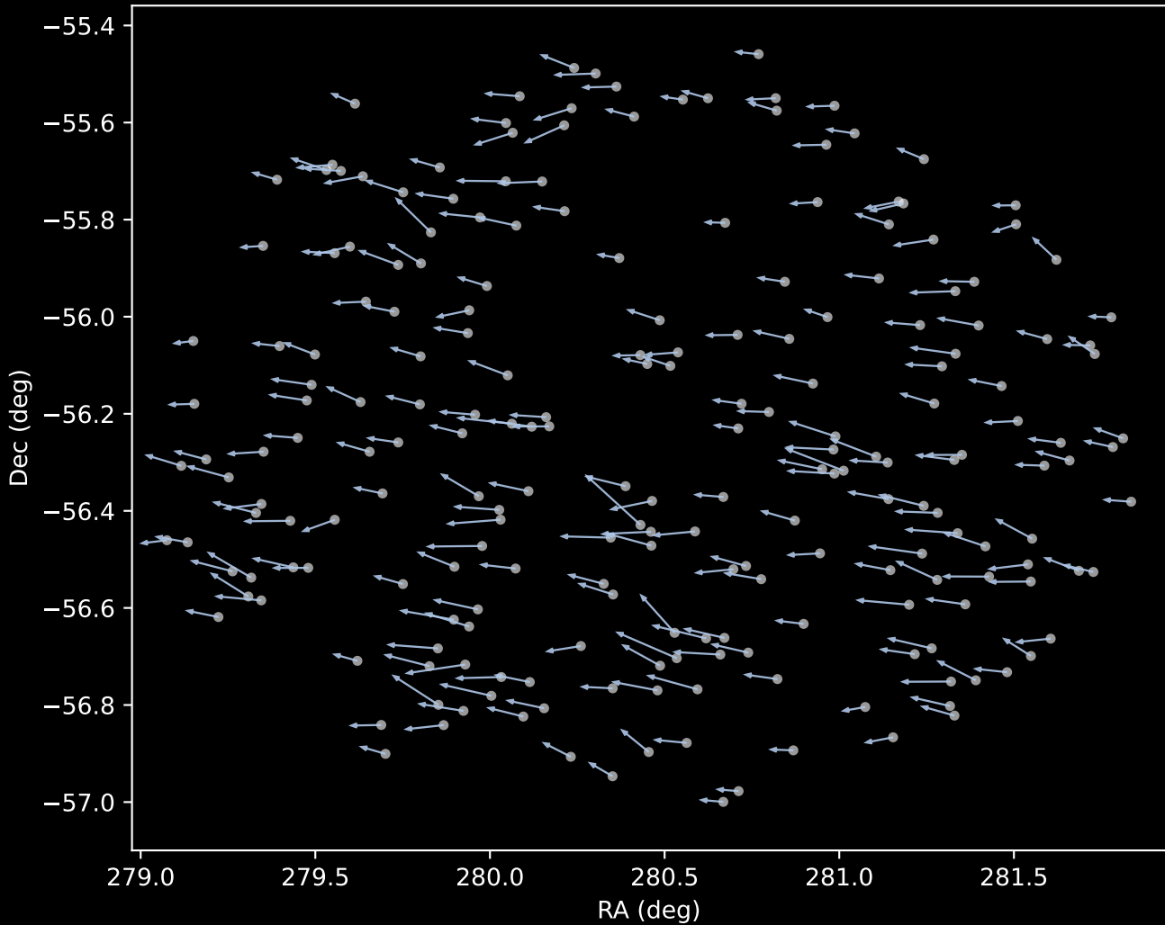
APOGEE DR17 Cluster 1 Proper Motion Vectors (n=219)
