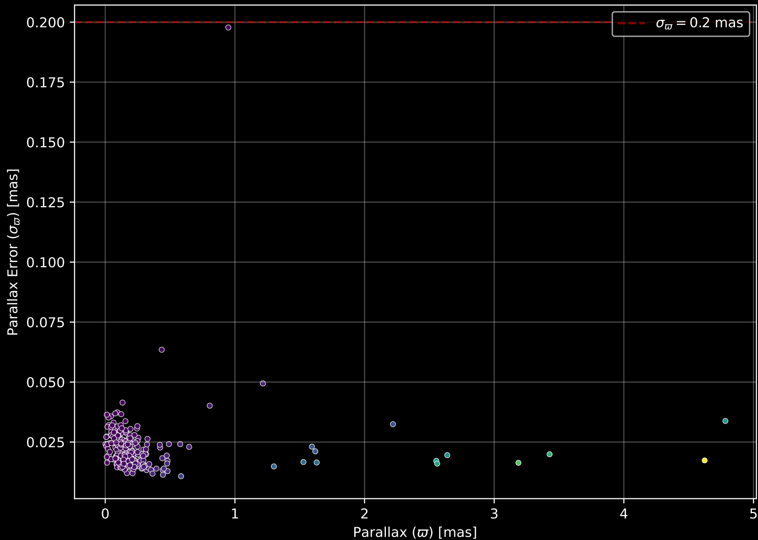
APOGEE DR17 Field: [296+06] Parallax Quality (n= 261)
