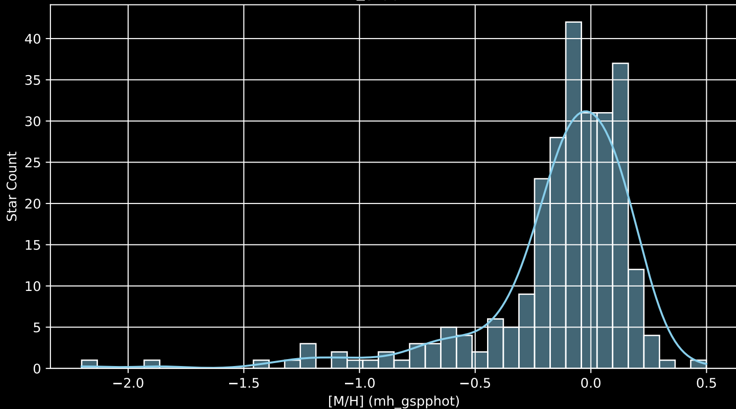
APOGEE DR17 Field: [296+06 [M/H] (mh_gspphot) (n= 261)
