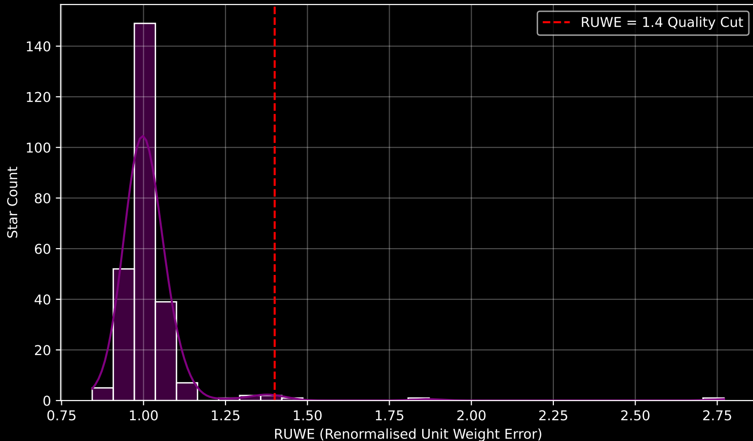
GAPOGEE DR17 Field [296+06] RUWE Distribution (n= 260)
