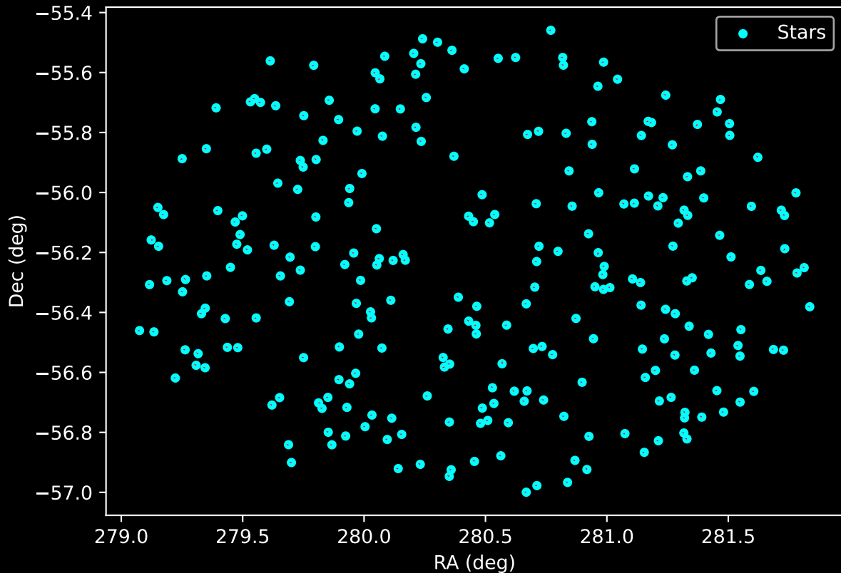
APOGEE DR17 Field: [296+06] Proper Motion Vectors for Gaia Star Field (n= 261)
