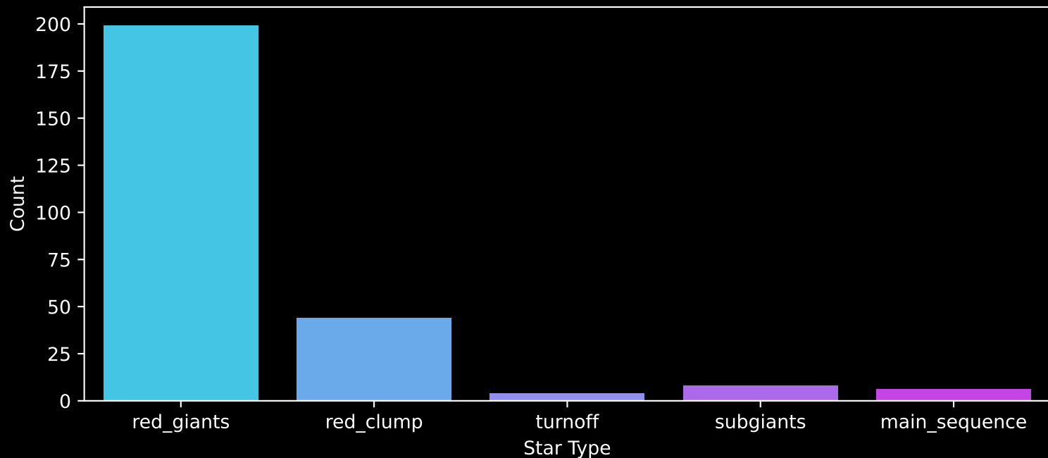
APOGEE DR17 Field: [296+06] Count plot of Star Type
